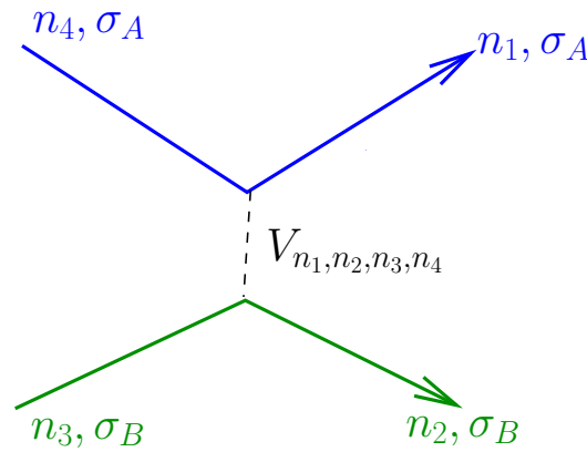
Figure 9.1: Interpretation of the interaction term in 9.42. Two particles in the initial levels n_3 and n_4 are scattered n_4 \rightarrow n_1 and n_3 \rightarrow n_2 . Spin is not changed by scattering, which explains the spin structure. In SQ scattering is described by first destroying the particles and then creating them in different levels. Also the matrix element in 9.42 (last line) can be understood by this picture
