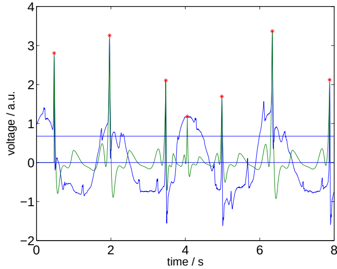
FIGURE 11. ECG signal with relative maxima and SR reference signal after applying step 6 of Signal Comparison Algorithm (SCA).
